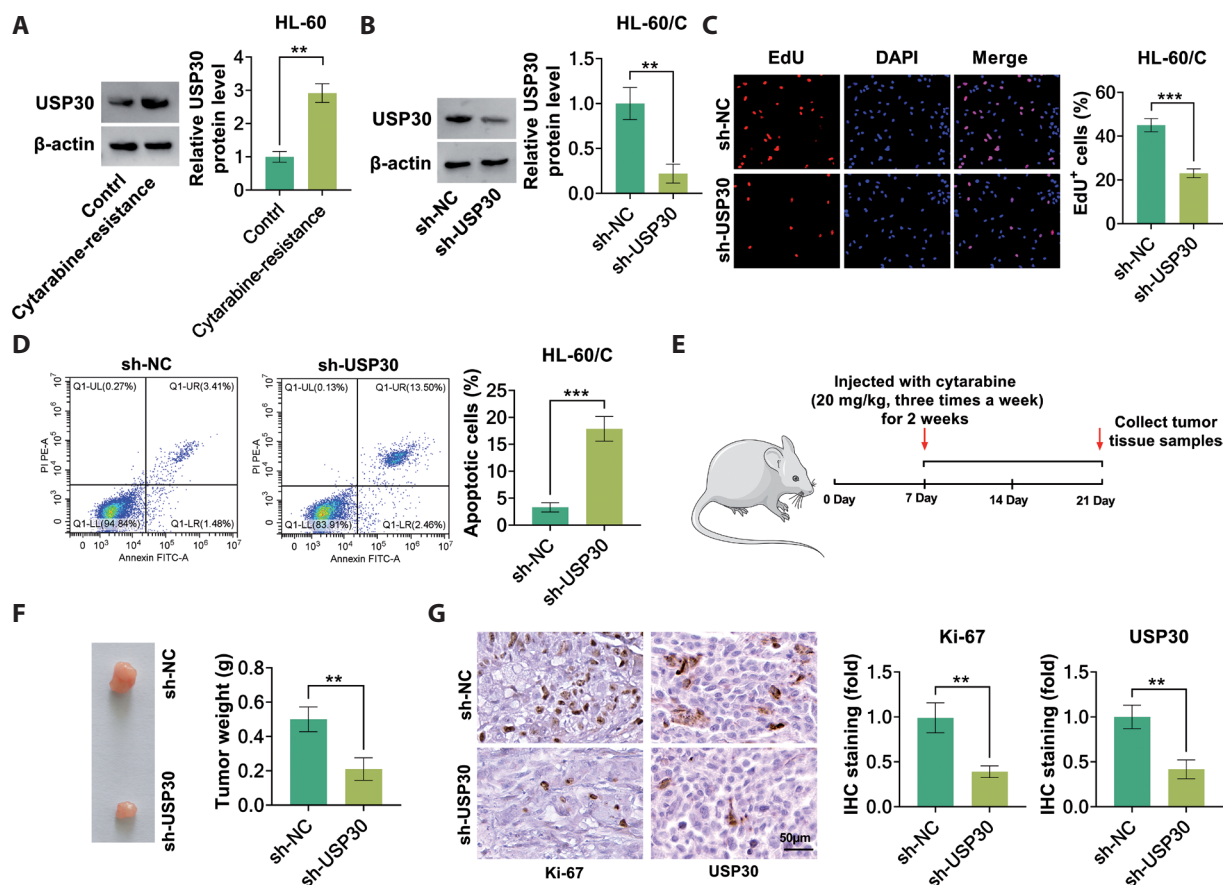
Figure 5. USP30 promotes Ara-C resistance in AML. A. USP30 expression in Ara-C-resistant HL-60 cells was determined by Western blot. B. Western blot analysis of USP30 protein level in HL-60/C cells transfected with sh-NC and sh-USP30. C. EdU assay was employed to assess cell proliferation of HL-60/C cells transfected with sh-NC and sh-USP30. D. Apoptosis of HL-60/C cells transfected with sh-NC and sh-USP30 was evaluated by flow cytometry. E-G. HL-60/C cells stably transfected with sh-NC and sh-USP30 were injected into BALB/c nude mice. From the 7 th day, these mice were injected with Ara-C (20 mg/kg) three times a week for 2 weeks. E. Animal treatment protocol schematic diagram. F. Tumor tissues were excised, photographed, and weighed. G. IHC was performed to assess the protein levels of Ki-67 and USP30 in tumor tissues. ** p < 0.01 , *** p < 0.001 .
