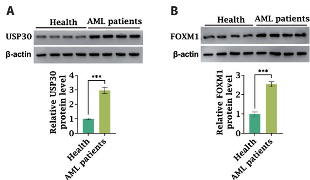
Figure 1. USP30 and FOXM1 expressions are upregulated in AML samples. USP30 (A) and FOXM1 (B) protein expression levels were detected by Western blot in bone marrow cells from healthy individuals ( n = 4 ) and AML patients ( n = 4 ). *** p < 0.001 .
