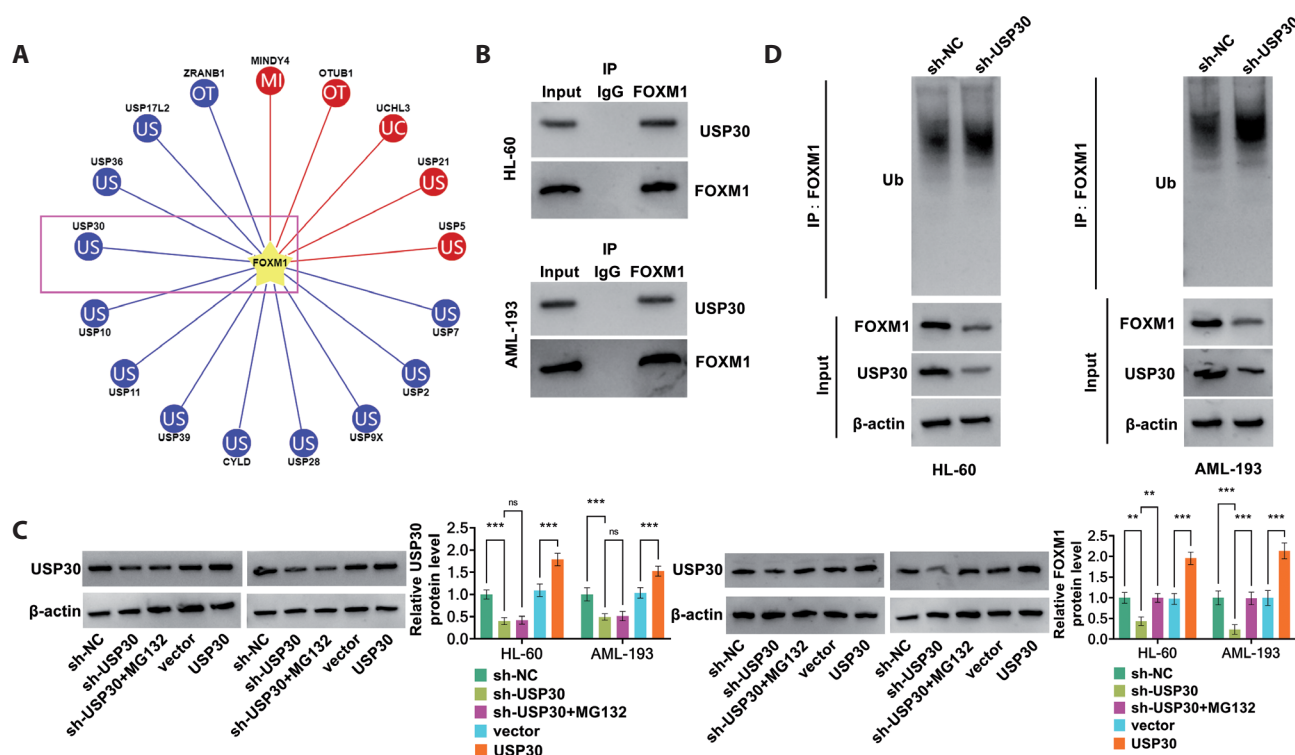
Figure 3. USP30 stabilizes FOXM1 expression via deubiquitination. A. The possible deubiquitination modification of USP30 on FOXM1 was predicted by UbiBrowser. B. Co-IP assay was used to detect the interaction between FOXM1 and USP30. C. HL-60 and AML-193 cells were treated with sh-NC, sh-USP30, sh-USP30+MG132, vector, and USP30. The protein levels of USP30 and FOXM1 were determined by Western blot. D. IP and Western blot were performed to analyze the ubiquitination level of FOXM1 in AML cells transfected with sh-NC and sh-USP30. ** p < 0.01 , *** p < 0.001 , ns, not significant.
